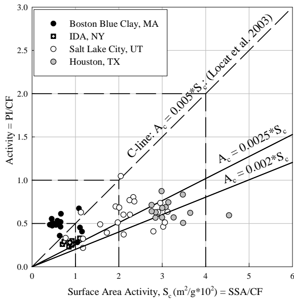
Figure 1. Relationship between Activity and Surface Area Activity.
