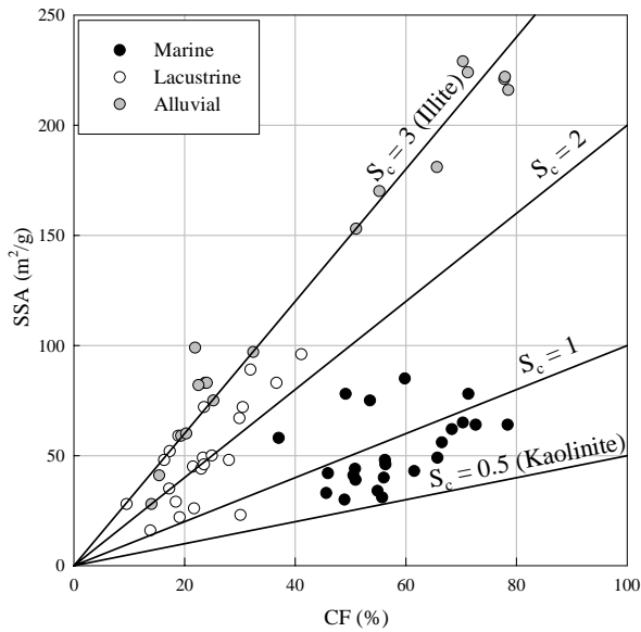
Figure 4. Surface Area Activity of Natural Clays.
