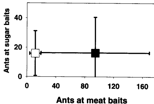
FIGURE 2. Average number of workers (SD) recruiting to meat and sugar baits in the canopy (dark square) and the litter (light square) after 32 min. Sugar baits attracted the same average number of ants in each habitat, while meat baits attracted more ants in the canopy.
