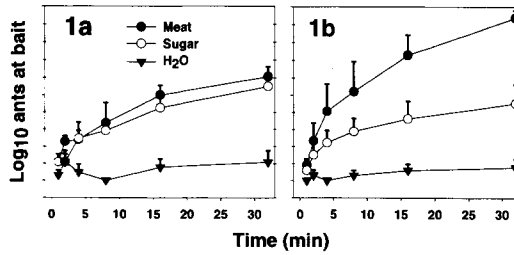
FIGURE 1. Results of choice experiments in the canopy and litter of the tropical tree Anacardium excelsum . Ant workers in the litter (1a) and canopy (1b) accumulated at different rates on three bait types. Roughly equal numbers of workers used sugar and meat baits in the litter; more workers used meat baits in the canopy. Vertical bars = 1 SE, N = 5 for each mean.
